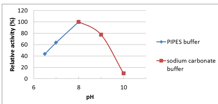
pH profile
